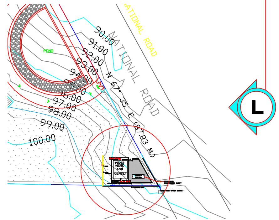
E 09 E TOPOGRAPHICAL LAYOUT REFERENCE 09 SCALE NTS
