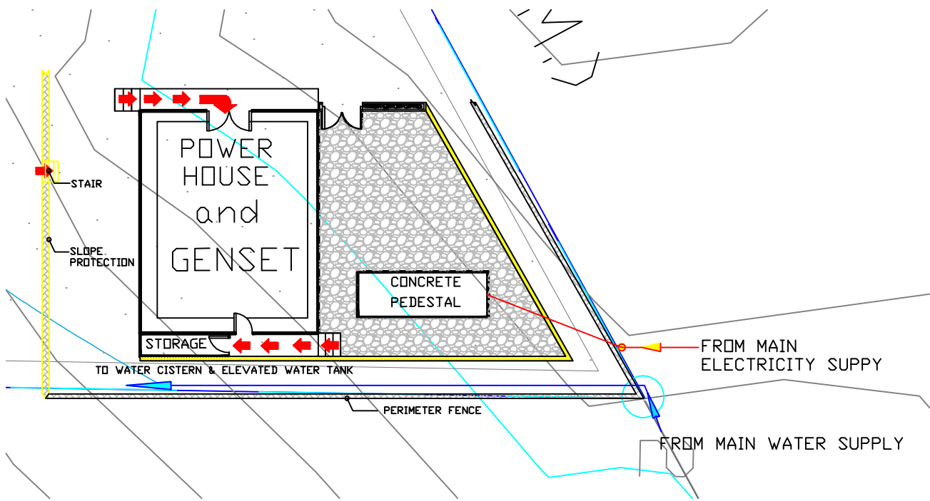
E 09 E TOPOGRAPHICAL LAYOUT REFERENCE 09 SCALE NTS
